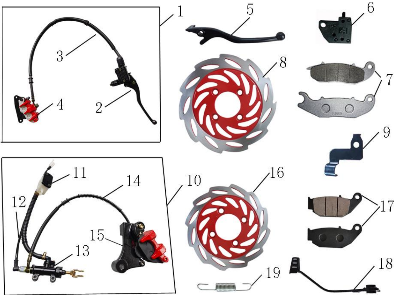
前后刹车系统 Front and rear braking system
