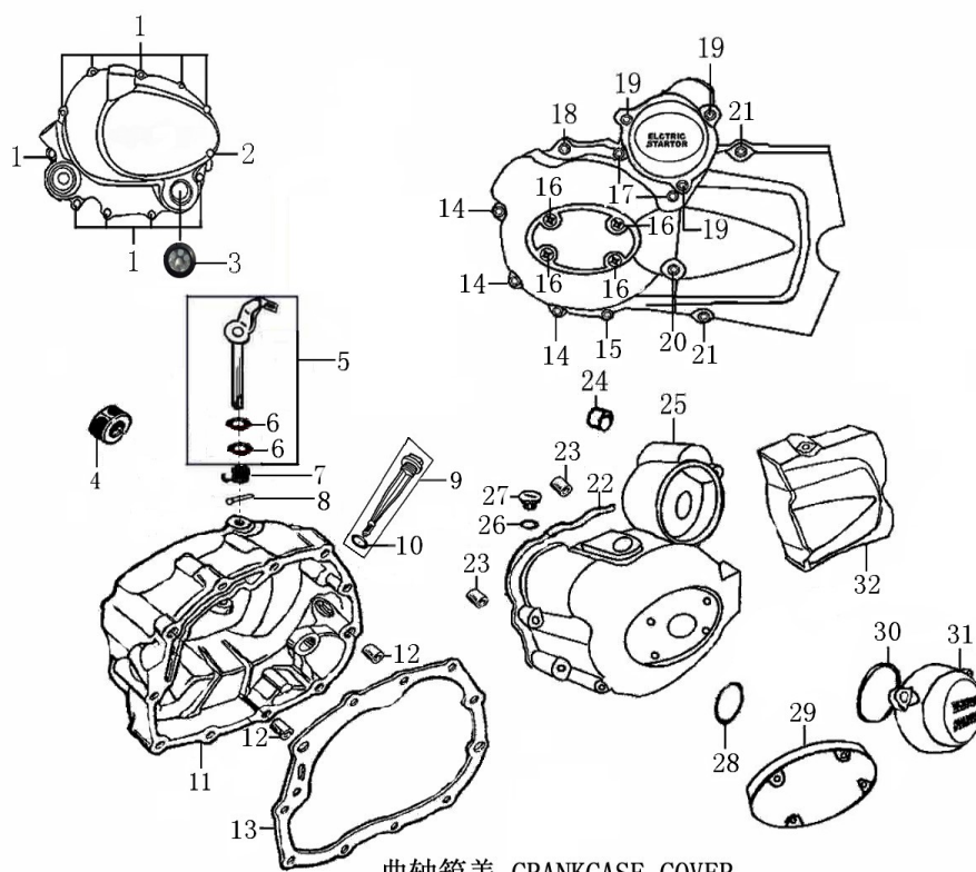
曲轴箱盖 CRANKCASE COVER
