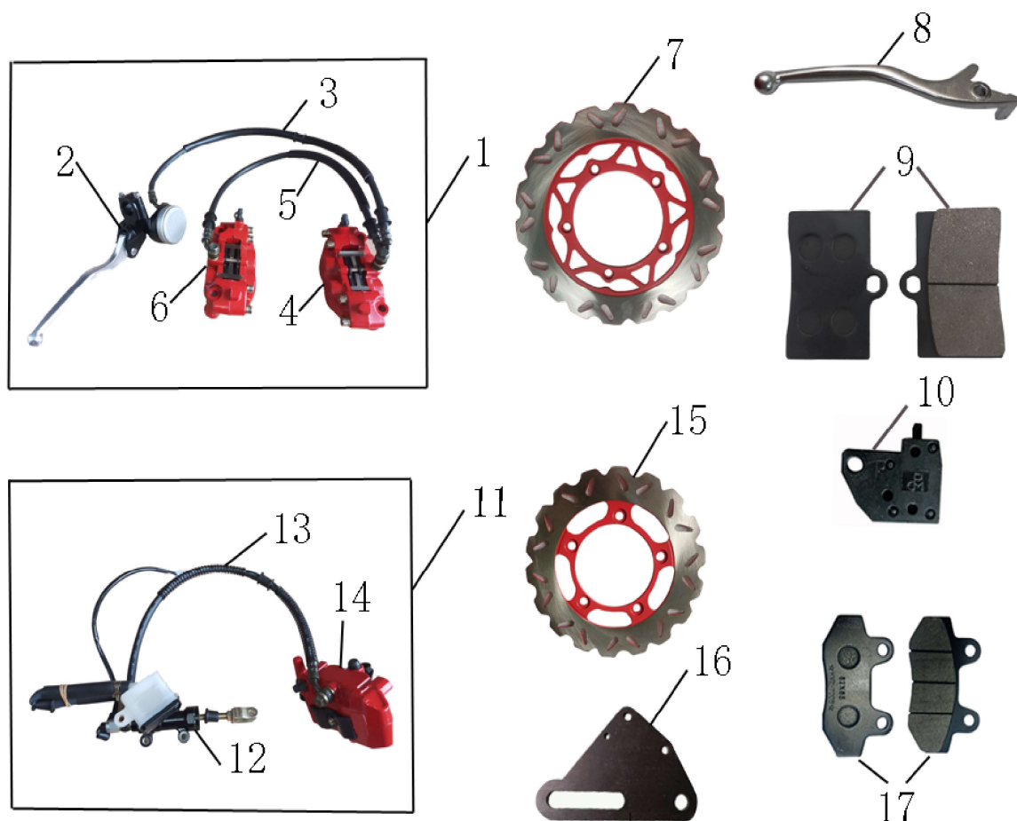
前后碟刹Front and rear brake system
