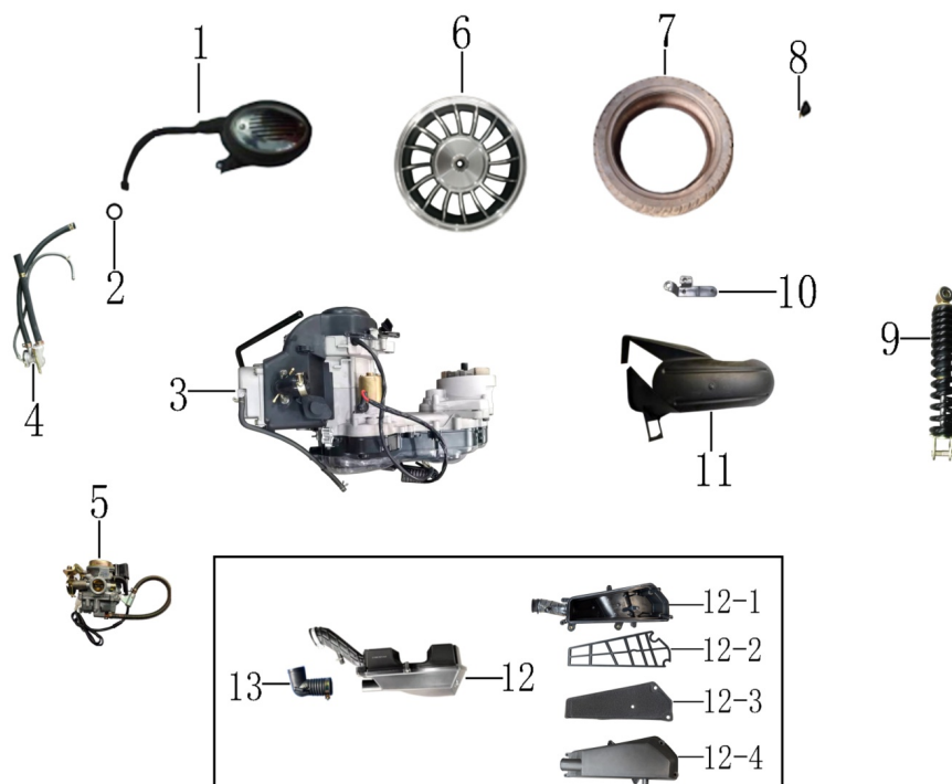
图8 发动机、化油器、消声器、空滤器、后轮及后减震 Engine, carburetor, muffler, air cleaner, rear wheel, rear shock absorber
