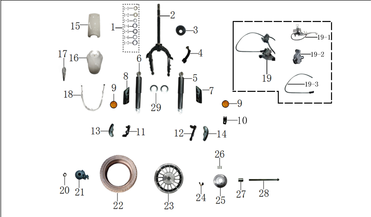
图4 前叉、前轮泥板、前减震、前碟刹泵及前轮总成 Front fork,front wheel fender,front shock absorber,front disc brake pump assy,front wheel assy
