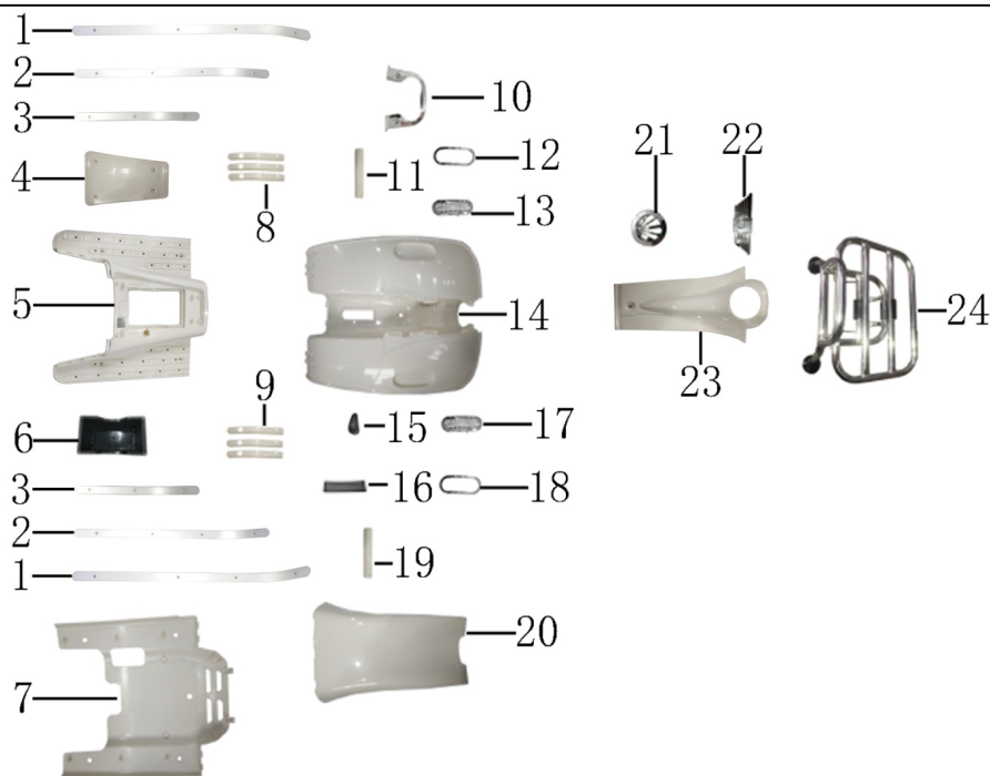
图2 前面板、前转向灯、脚踏板、车架挡泥板及前载物架 Front panel, fron turn signal, footrest, frame fender&front carrier
