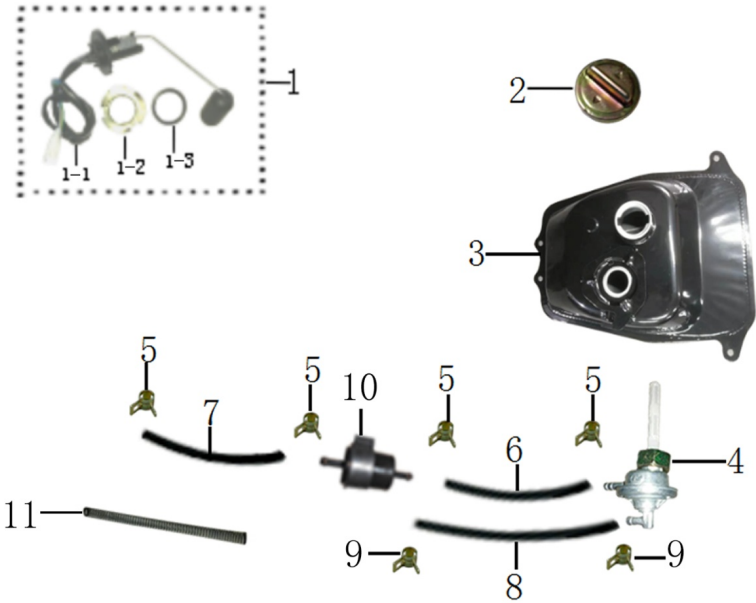
图6 油箱、燃油传感器、油管、燃油过滤器、油开关 tank, fuel sensor, fuel hose, fuel filter, fuel pump
