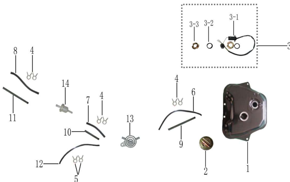
图5 油箱、燃油传感器、油管、燃油过滤器、负压开关 tank, fuel sensor, fuel pipe, fuel filter, fuel pump
