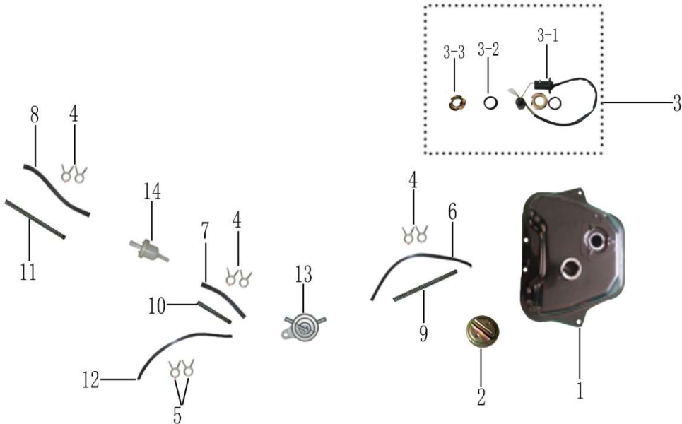
图5 油箱、燃油传感器、油管、燃油过滤器、负压开关 tank, fuel sensor, fuel pipe, fuel filter, fuel pump
