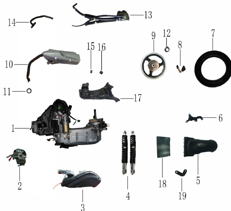
图7 发动机、化油器、消声器、后轮及后减震 Engine, carburetor, muffler, rear wheel and rear shock absorber
