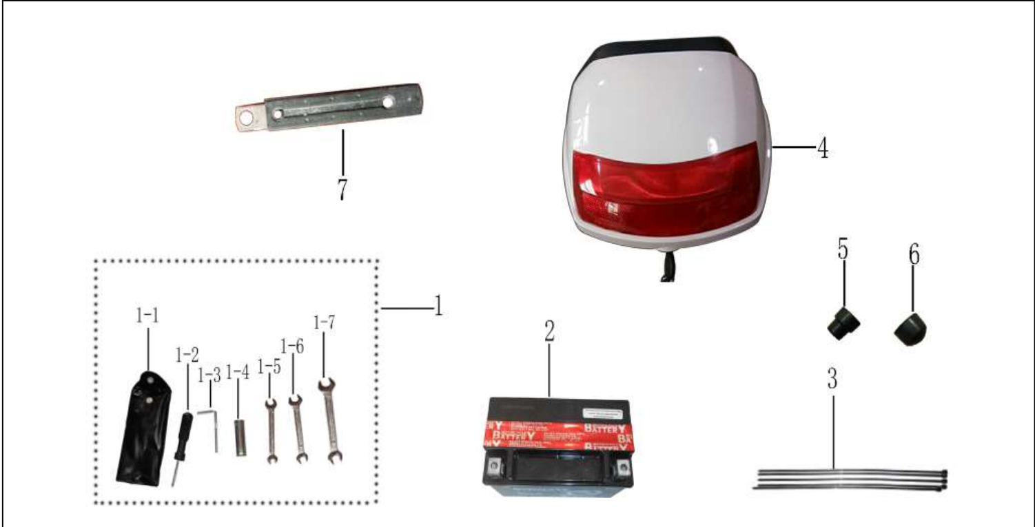
图8 随车工具包、蓄电池、扎带、尾箱 kit, battery, belting, footrest rubber Tool
