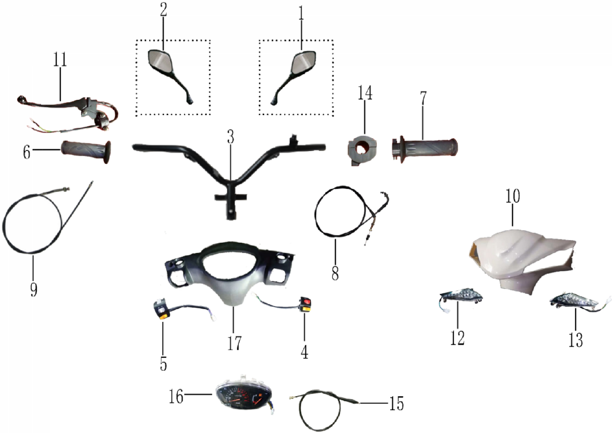
图1后视镜、方向把、头罩前后部及仪表总成、前左右转向灯 Rearview mirror, handlebar assy, head hood & speedometer assy, front turning signal
